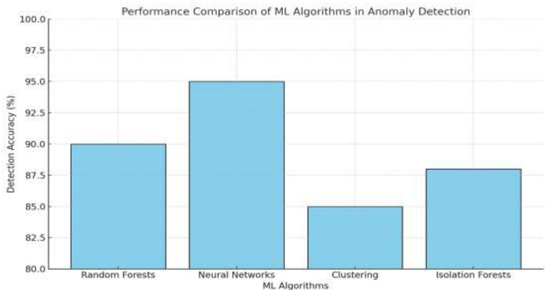
Graph: Performance Comparison of ML Algorithms in Anomaly Detection
